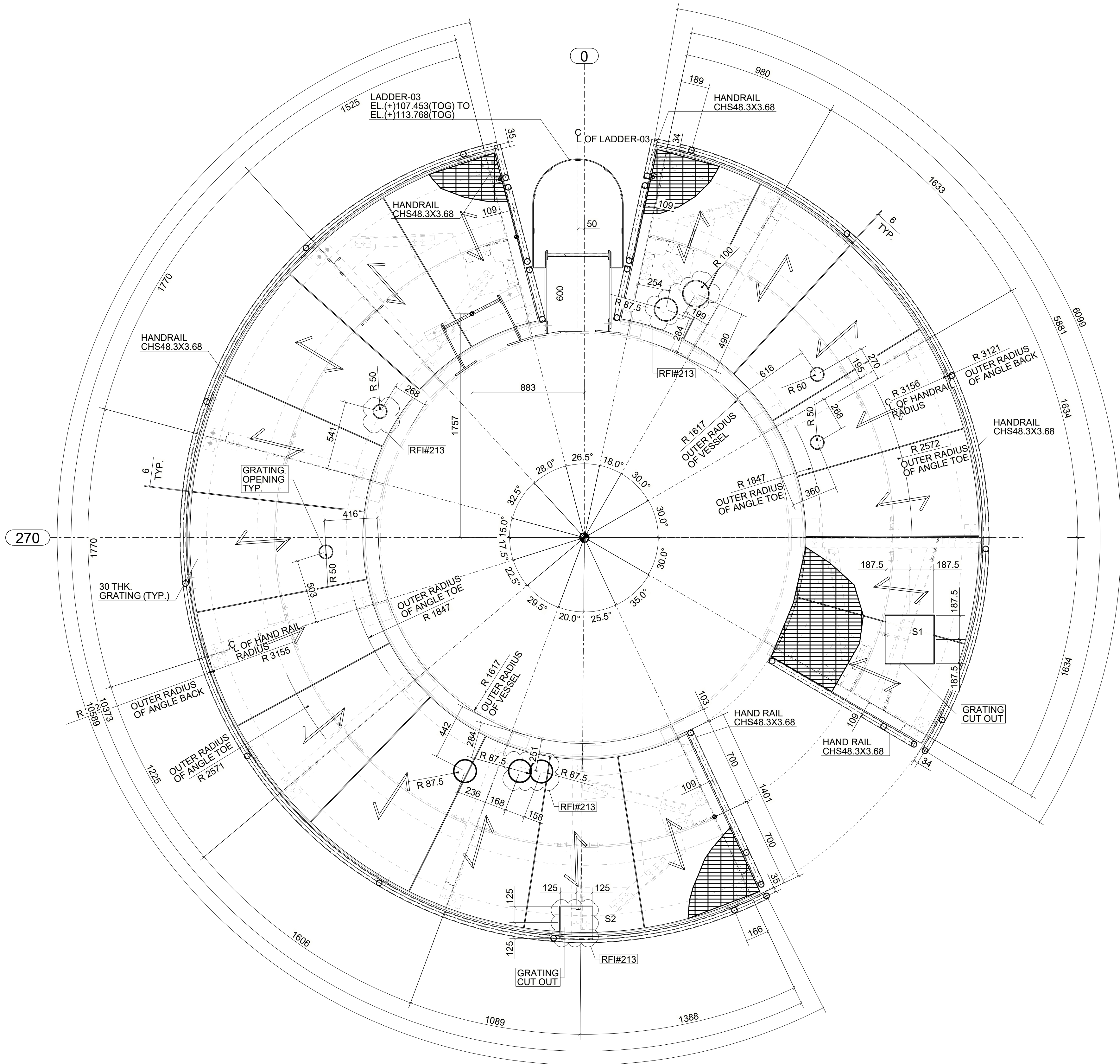
GRATING & HANDRAIL PLAN AT EL. + 113.768 (TOG) ALL PLAN BRACING ARE AT (-50) UNO
