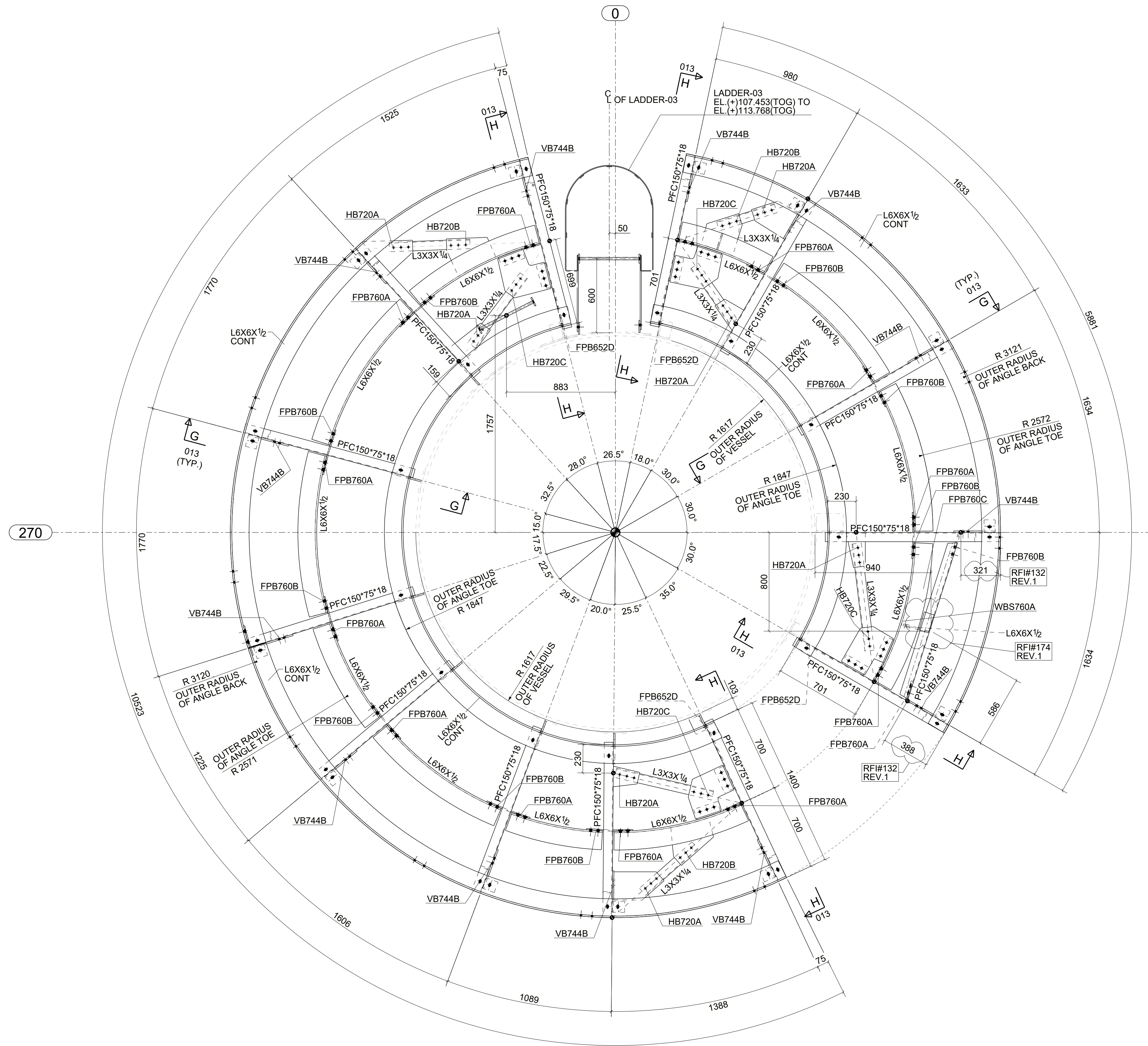
PLATFORM FRAMING PLAN AT EL. + 113.725 (TOS) ALL PLAN BRACING ARE AT (-50) UNO
