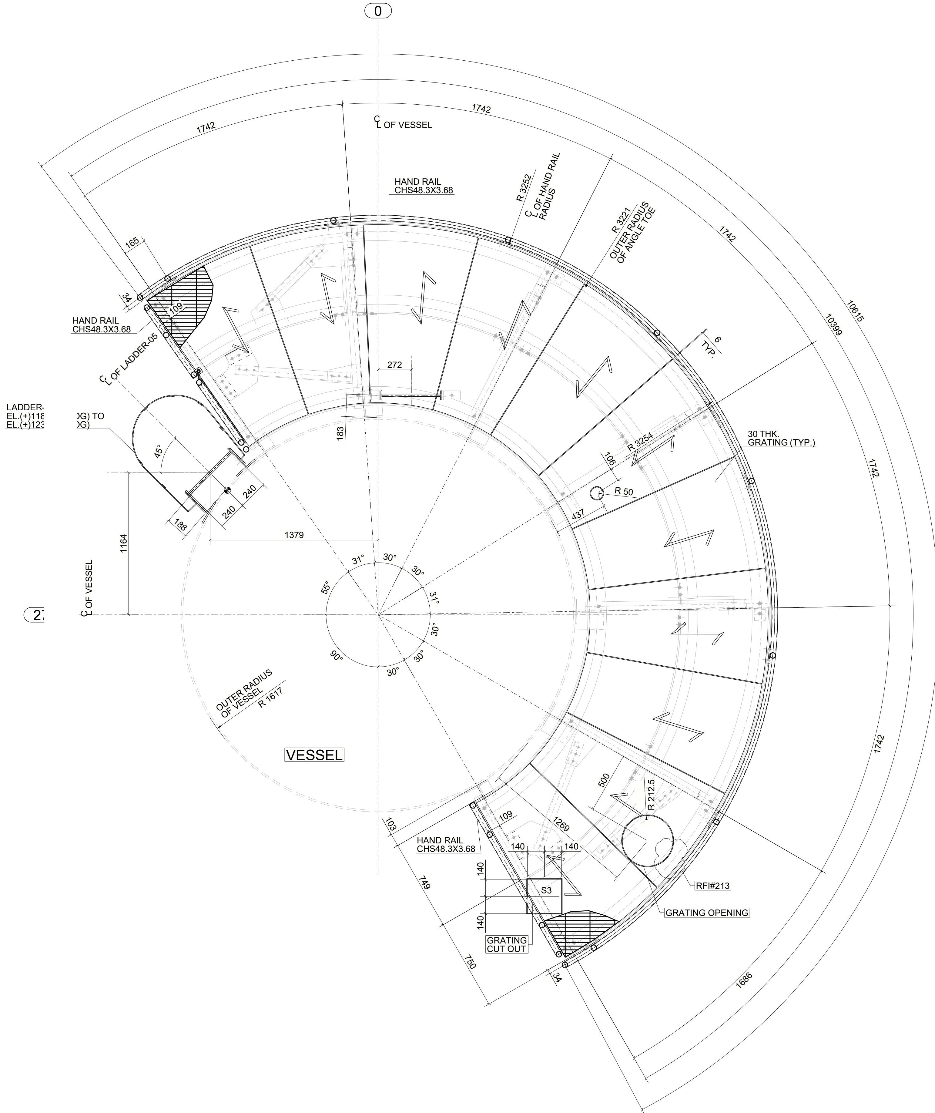
GRATING & HANDRAIL PLAN AT EL.+123.418 (TOG) ALL PLAN BRACING ARE AT (-50) UNO
